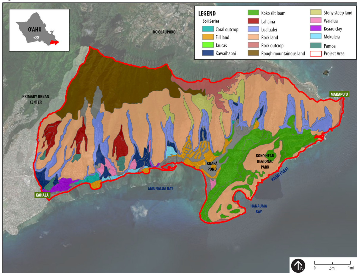
Figure 2-8: East Honolulu Soil Series
