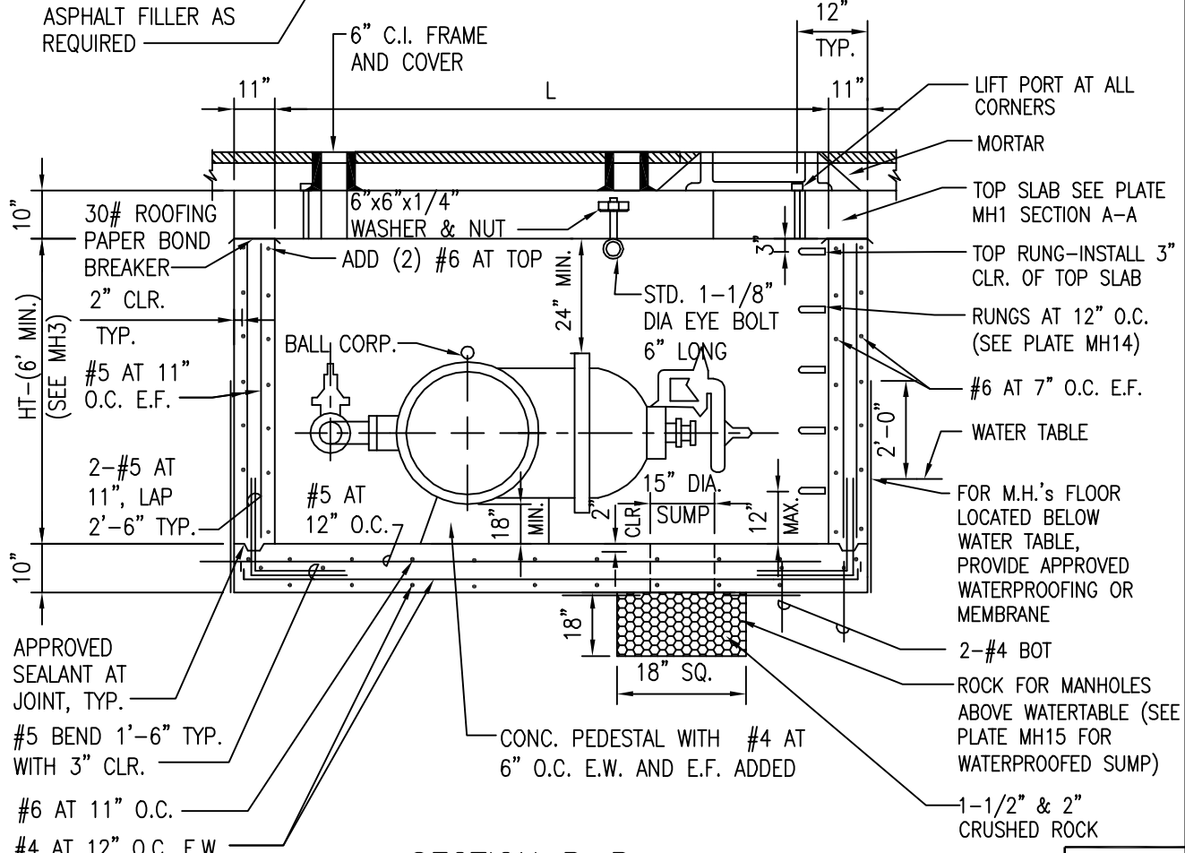
SECTION B-B CAST-IN-PLACE WALL
