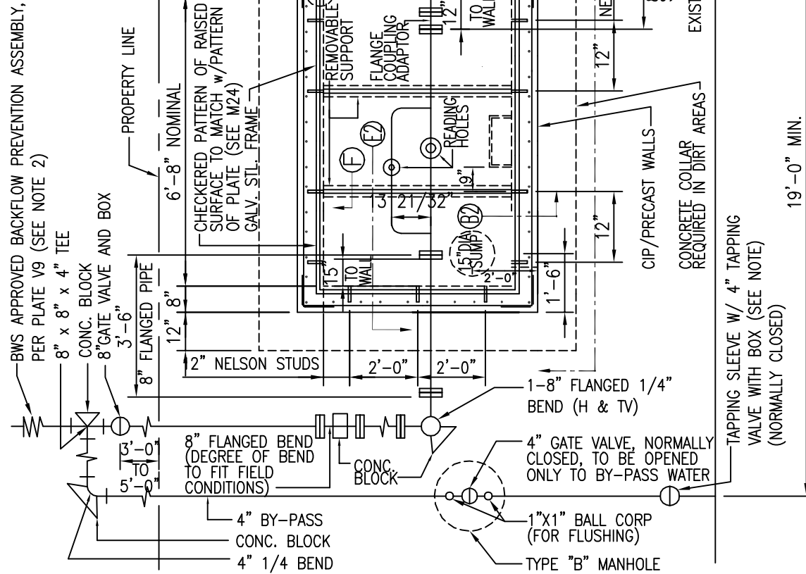
PLAN VIEW OF GALV. STEEL FRAME AND REMOVABLE SUPPORT PRECAST/CAST IN PLACE WALLS
