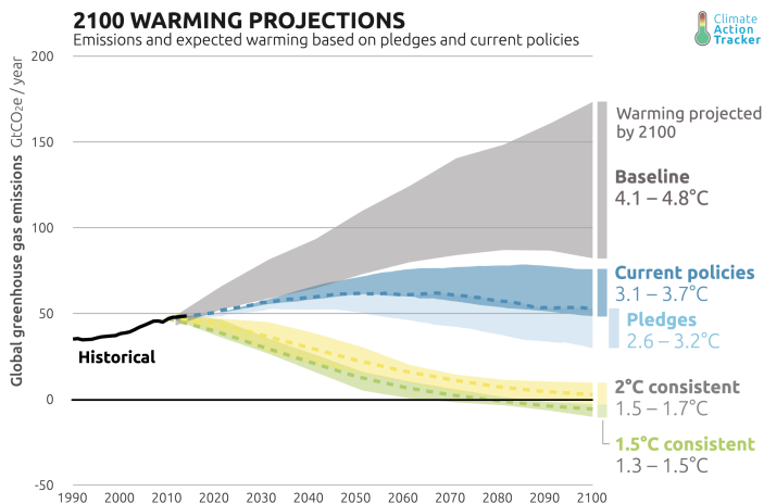
Figure 4. Although some large emitters, including China, the EU and India have either reduced—or slowed—their GHG emissions growth rate, currently implemented policies are expected to result in a further growth of global GHG emissions by about 9–13% between 2020–2030. Source: Climate Action Tracker: https://climateactiontracker.org/publications/improvement-warming-outlook-india-and-china-move-ahead-paris-agreement-gap-still-looms-large/
