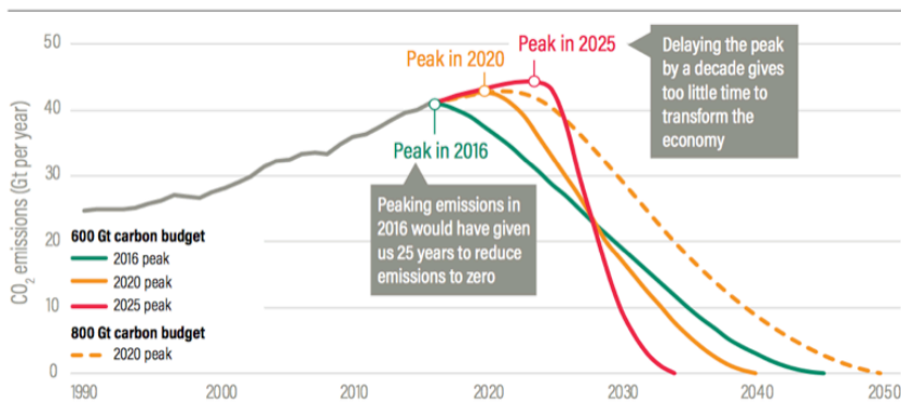
Figure 2. Climate models indicate that the world can stop global warming at 2°C if greenhouse gas emissions are reduced by 50% per decade immediately. Delaying this reduction leads to warming of more than 3°C – a dangerous level. Source: Levin, K., and Rich, D. (2017) Turning Points: Trends in Countries' Reaching Peak Greenhouse Gas Emissions over Time . Working Paper. Washington, DC: World Resources Institute. Available online at http://www.wri.org/publication/turning-points .
