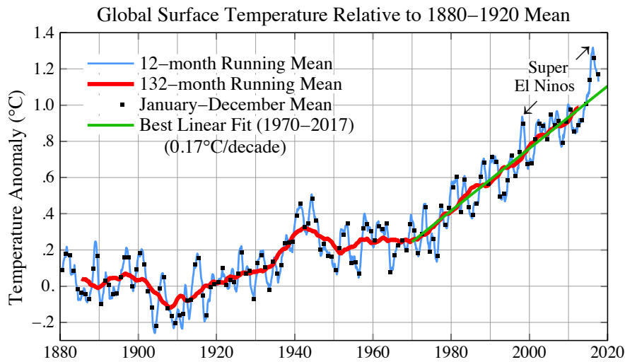
Figure 1. Global temperature since 1880. In 1970 global surface temperature began a consistent, long-term rise at a rate of 0.3°F (0.17°C) per decade. Individual years, or groups of years, may be warmer or cooler than this trend due to various causes of climate variability. These include cooling effects from light scattering particles in the atmosphere (e.g., sulfur aerosols from volcanic and industrial emissions), the El Niño Southern Oscillation, the Pacific Decadal Oscillation, and others.
