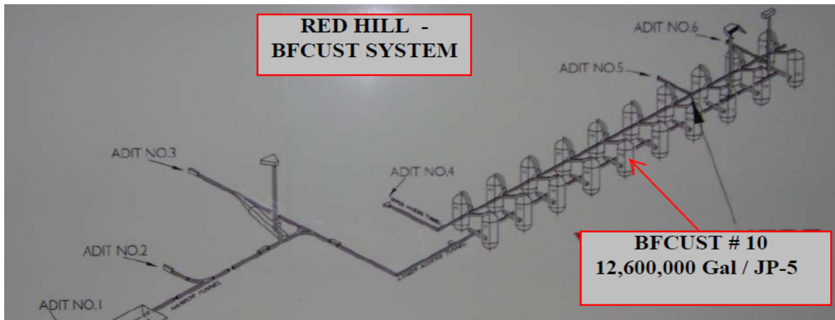
Figure 1: RED HILL – BFCUST SYSTEM – BFCUST #10
